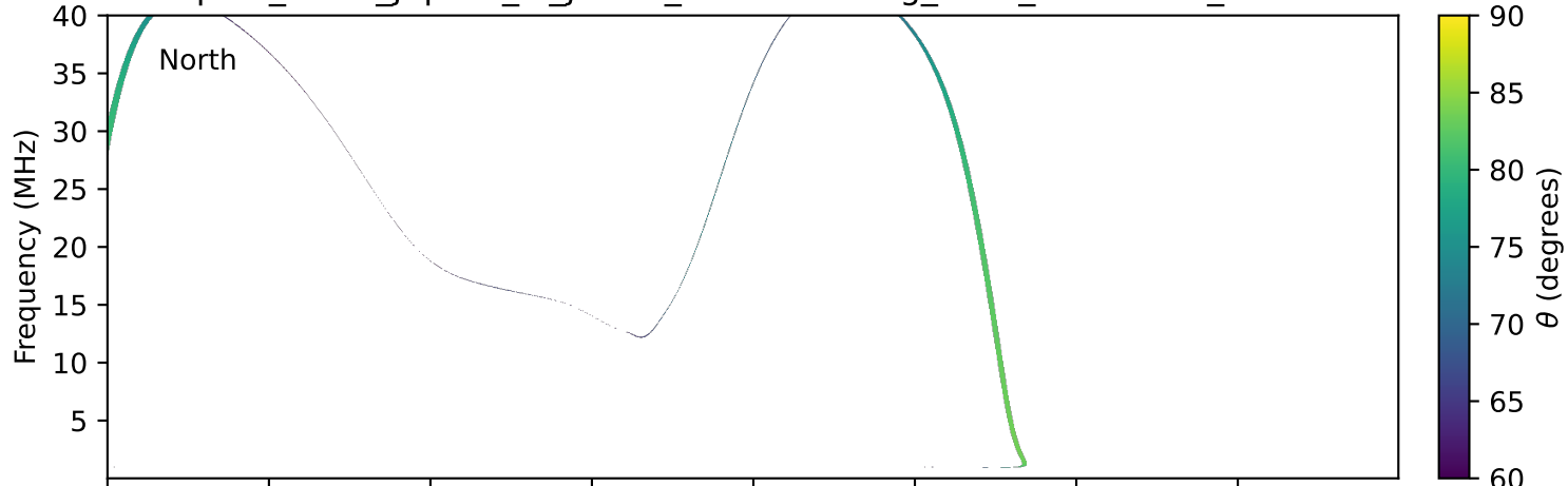
expres_earth_jupiter_io_jrm09_lossc-wid1deg_3kev_19921207_v11.cdf
