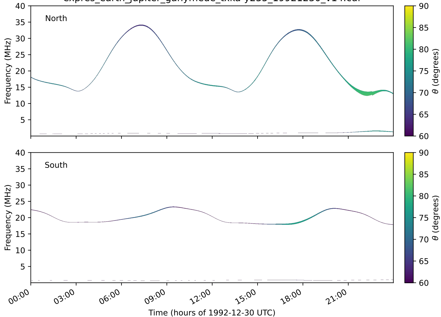
expres_earth_jupiter_ganymede_txka-y235_19921230_v14.cdf
