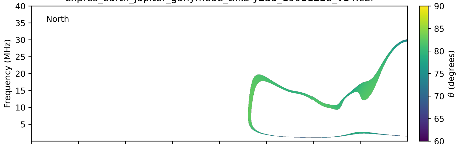
expres_earth_jupiter_ganymede_txka-y235_19921228_v14.cdf
