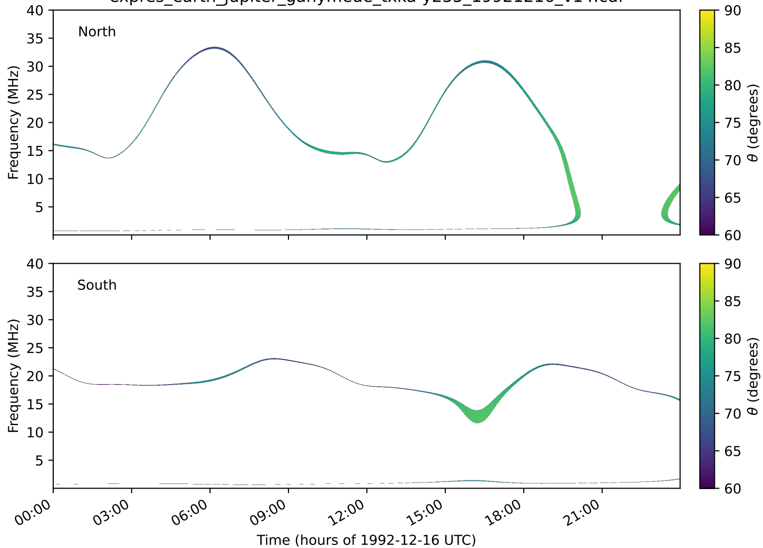
expres_earth_jupiter_ganymede_txka-y235_19921216_v14.cdf
