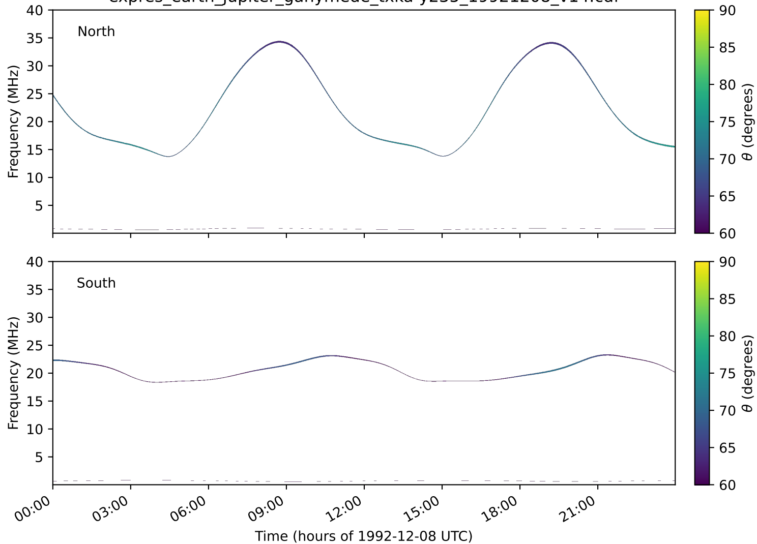
expres_earth_jupiter_ganymede_txka-y235_19921208_v14.cdf
