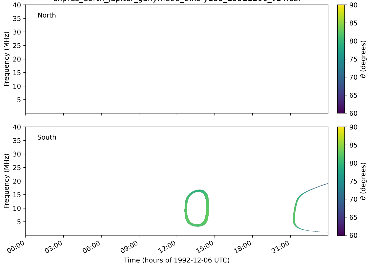
expres_earth_jupiter_ganymede_txka-y235_19921206_v14.cdf
