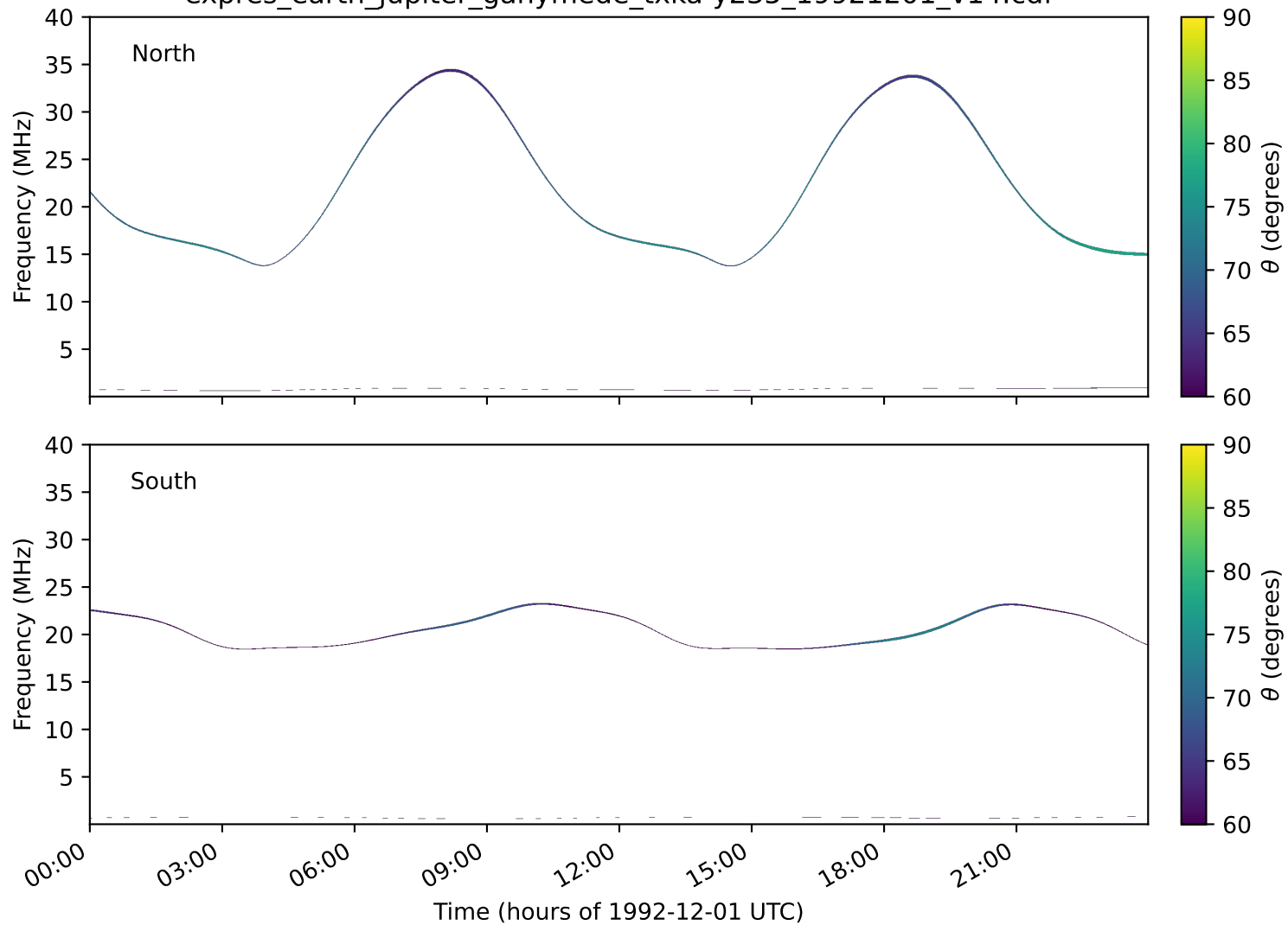
expres_earth_jupiter_ganymede_txka-y235_19921201_v14.cdf
