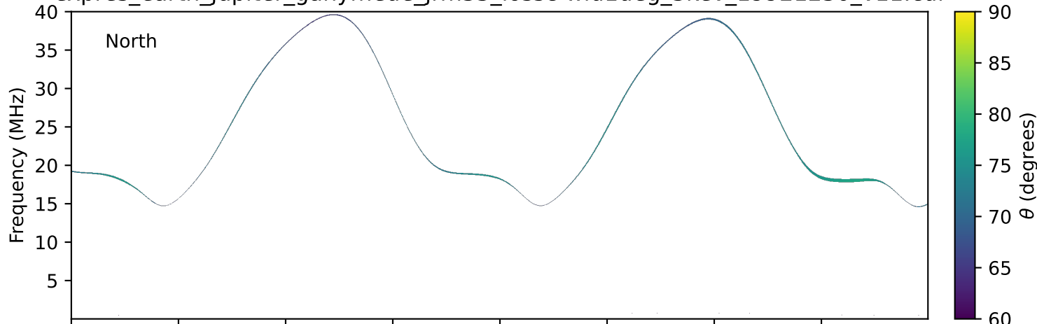
expres_earth_jupiter_ganymede_jrm33_lossc-wid1deg_3kev_19921230_v11.cdf
