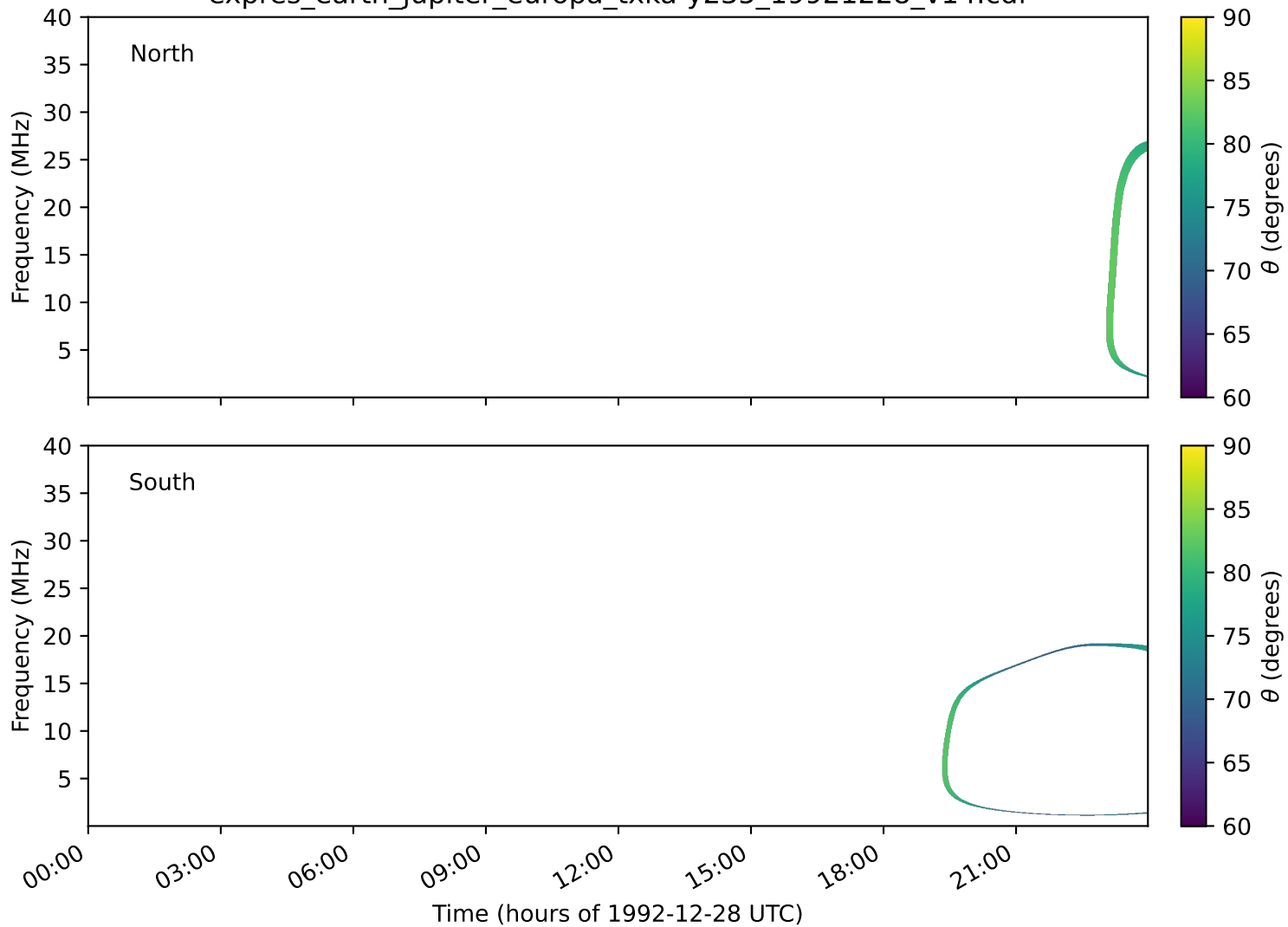
expres_earth_jupiter_europa_txka-y235_19921228_v14.cdf
