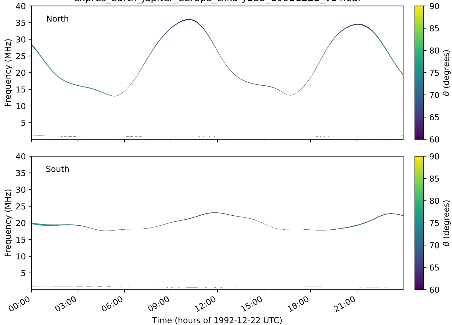
expres_earth_jupiter_europa_txka-y235_19921222_v14.cdf
