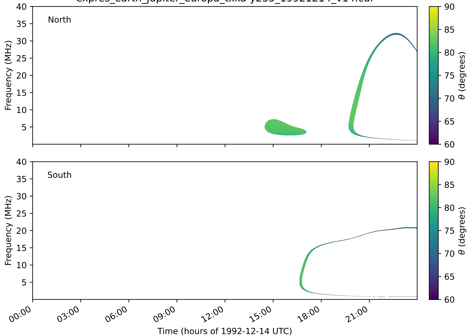
expres_earth_jupiter_europa_txka-y235_19921214_v14.cdf
