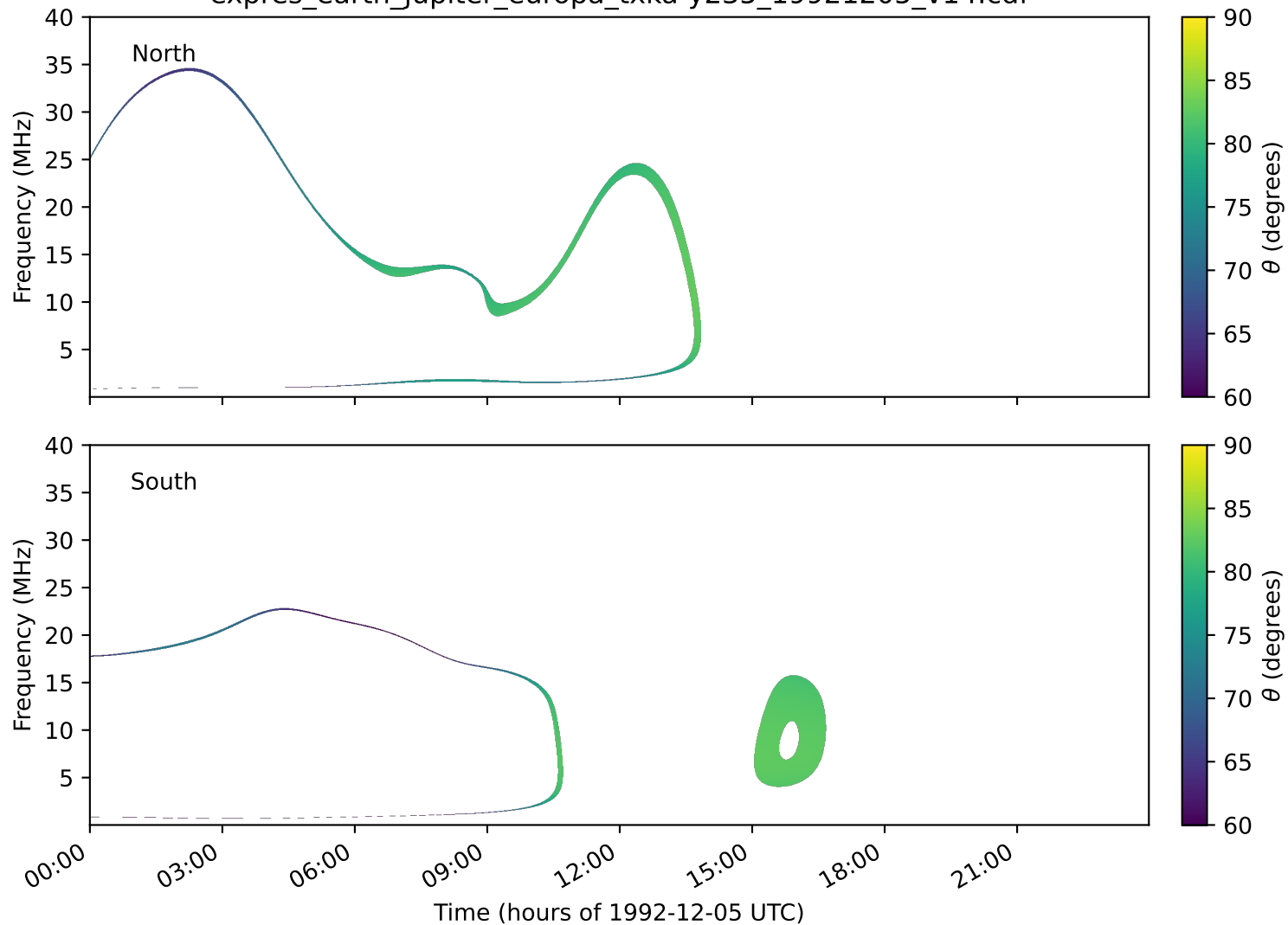
expres_earth_jupiter_europa_txka-y235_19921205_v14.cdf
