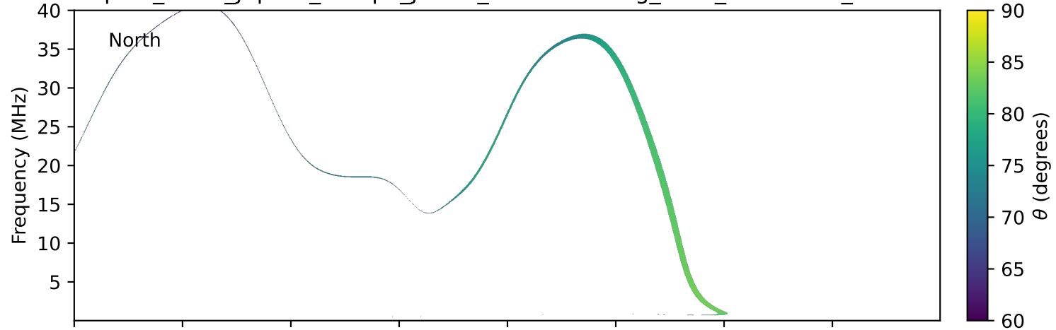
expres_earth_jupiter_europa_jrm33_lossc-wid1deg_3kev_19921219_v11.cdf
