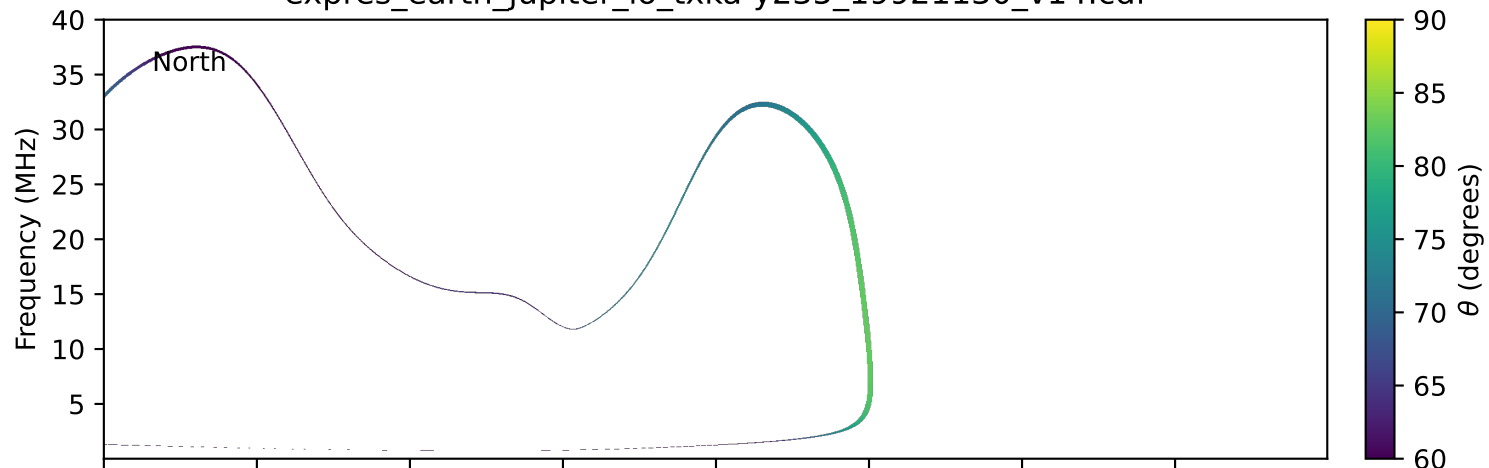
expres_earth_jupiter_io_txka-y235_19921130_v14.cdf
