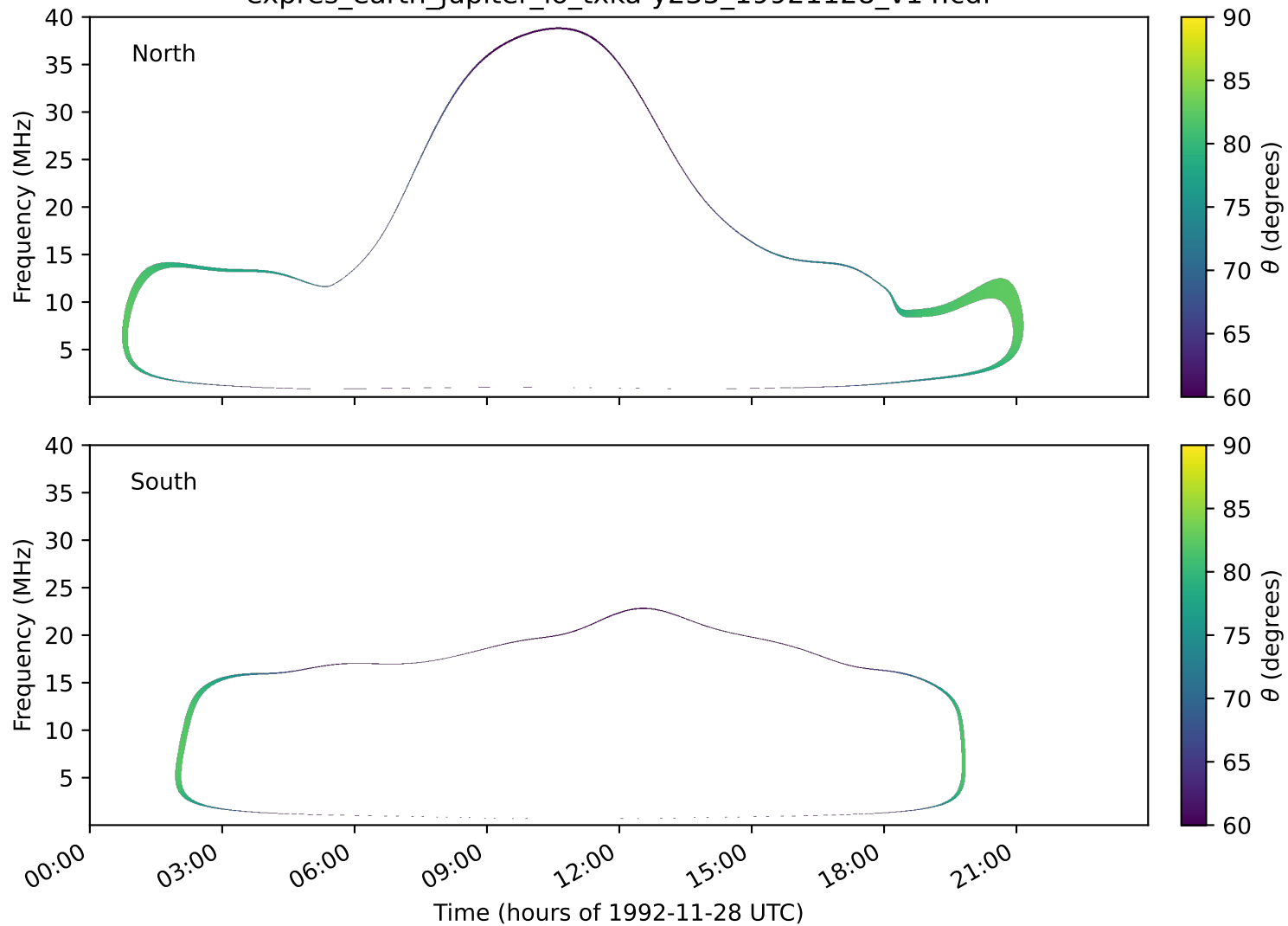
expres_earth_jupiter_io_txka-y235_19921128_v14.cdf
