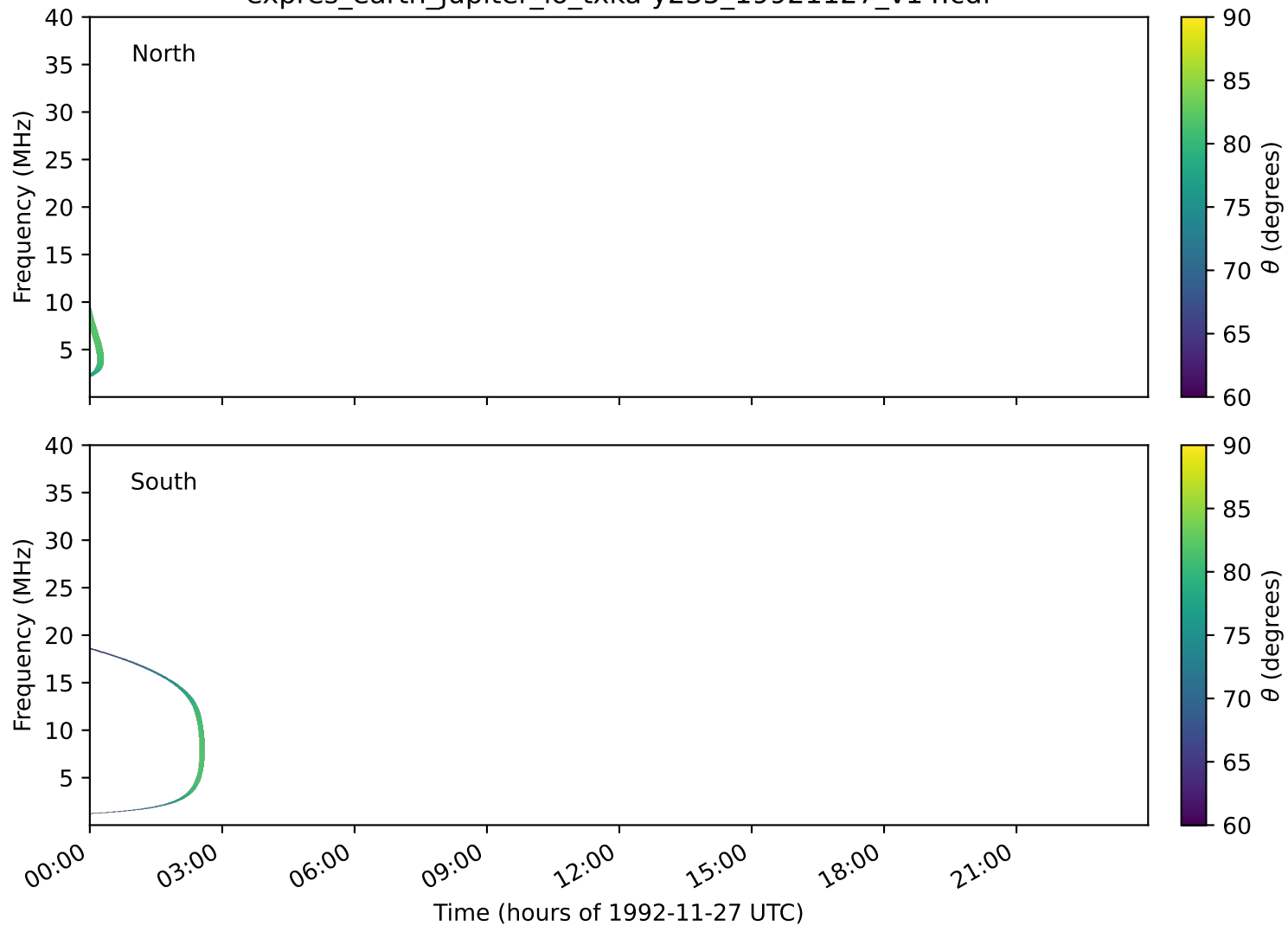
expres_earth_jupiter_io_txka-y235_19921127_v14.cdf
