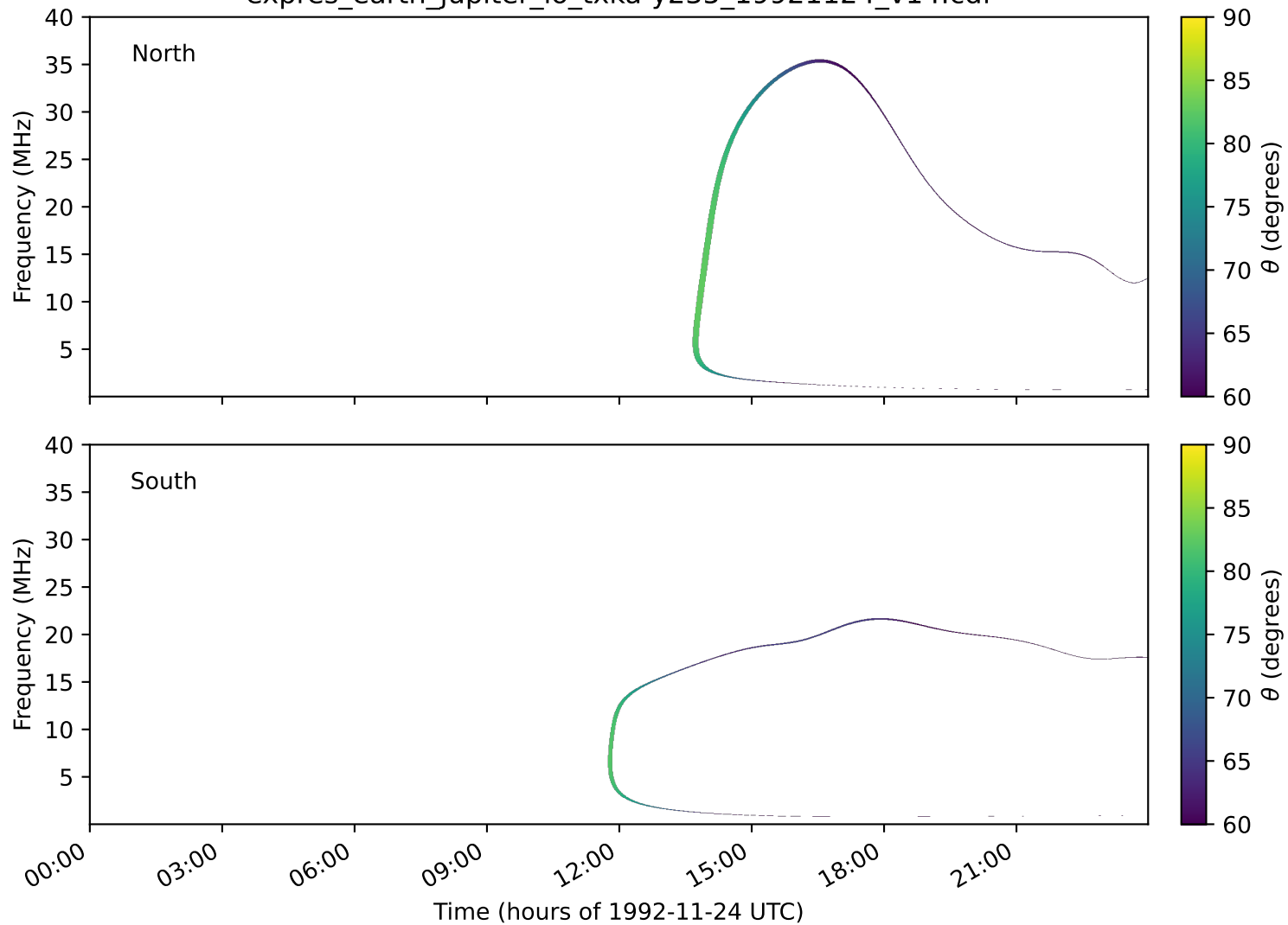
expres_earth_jupiter_io_txka-y235_19921124_v14.cdf
