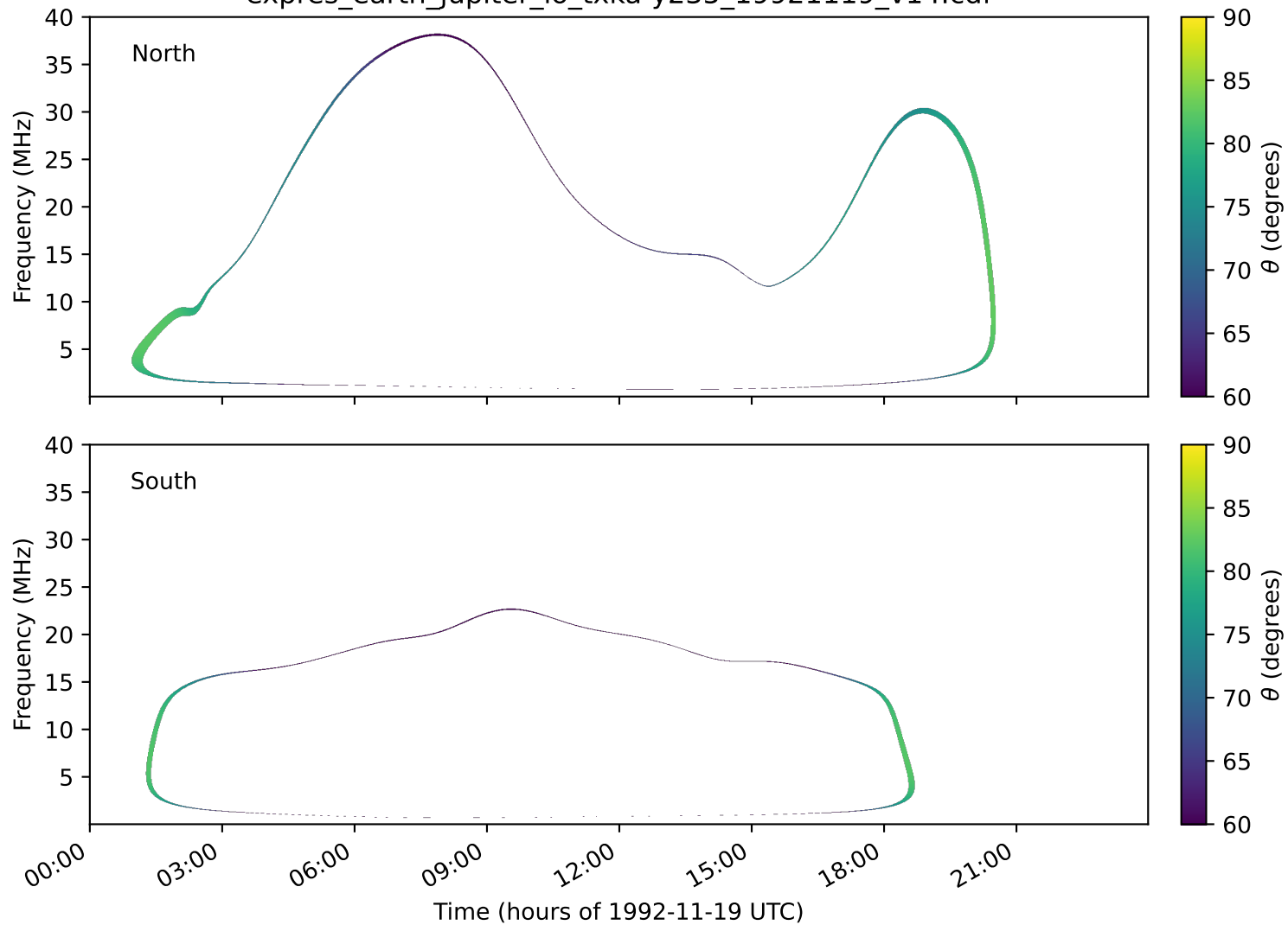
expres_earth_jupiter_io_txka-y235_19921119_v14.cdf
