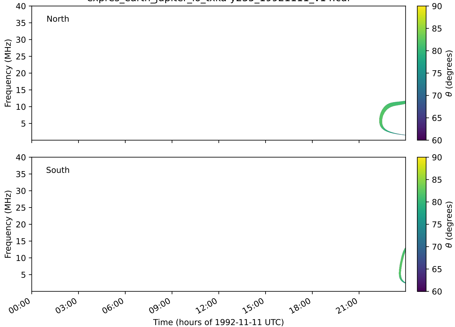
expres_earth_jupiter_io_txka-y235_19921111_v14.cdf
