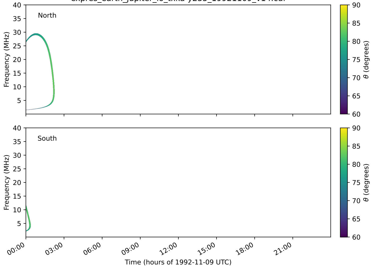
expres_earth_jupiter_io_txka-y235_19921109_v14.cdf
