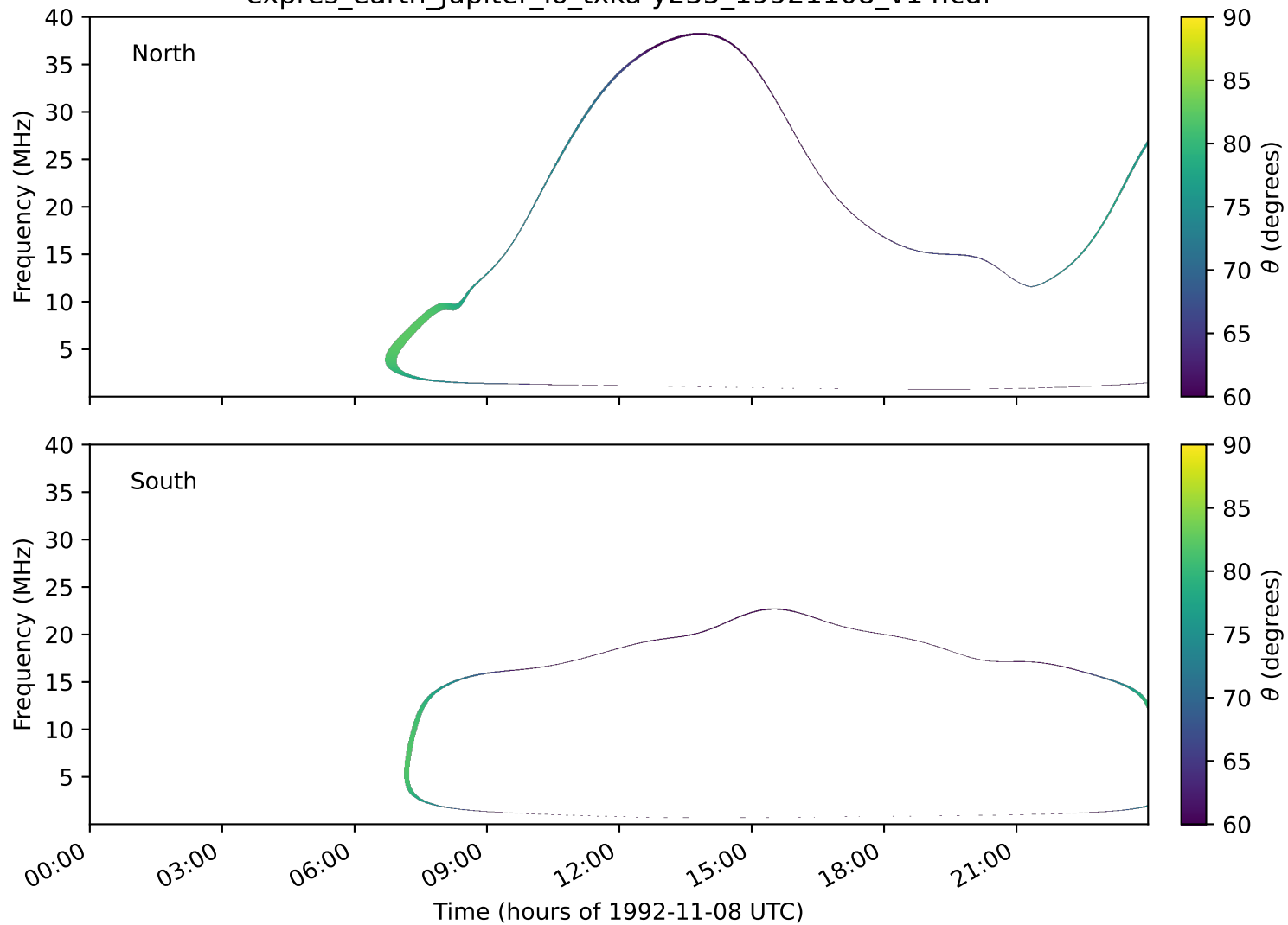
expres_earth_jupiter_io_txka-y235_19921108_v14.cdf
