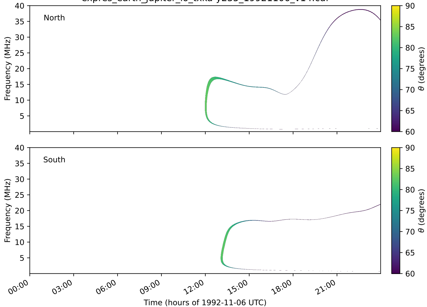
expres_earth_jupiter_io_txka-y235_19921106_v14.cdf
