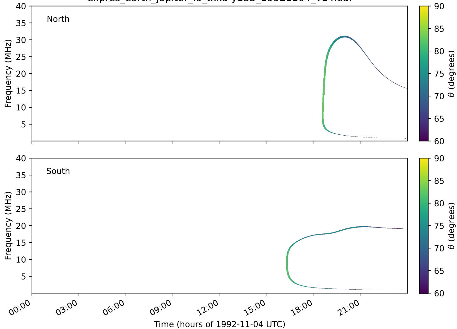
expres_earth_jupiter_io_txka-y235_19921104_v14.cdf
