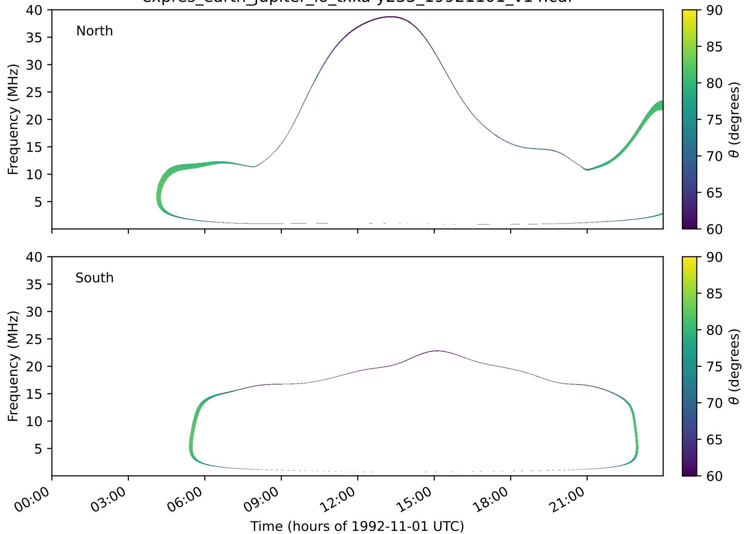
expres_earth_jupiter_io_txka-y235_19921101_v14.cdf
