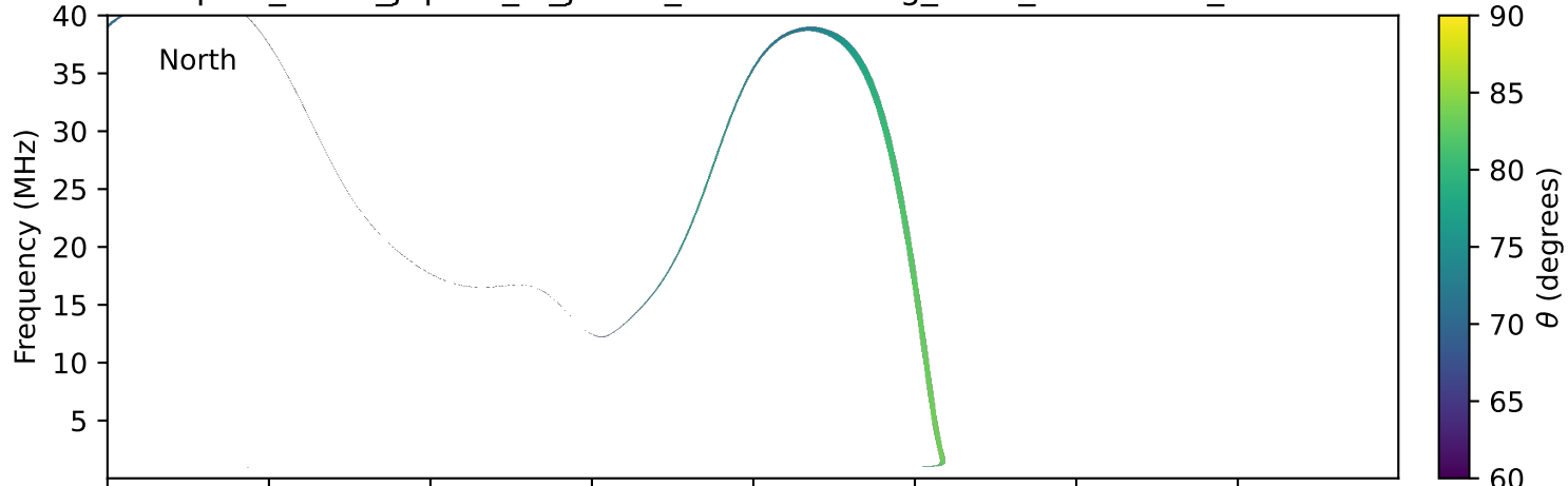
expres_earth_jupiter_io_jrm33_lossc-wid1deg_3kev_19921130_v11.cdf
