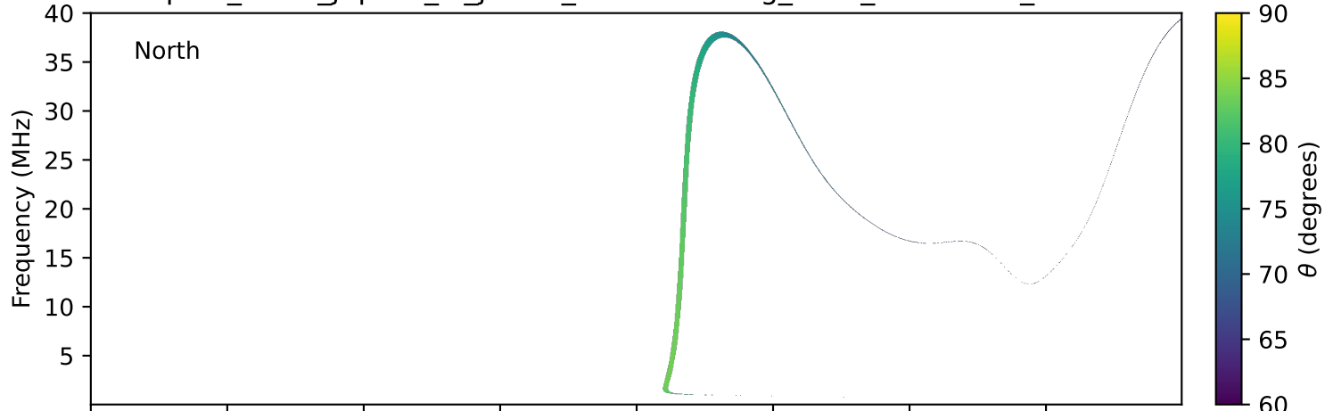
expres_earth_jupiter_io_jrm33_lossc-wid1deg_3kev_19921115_v11.cdf
