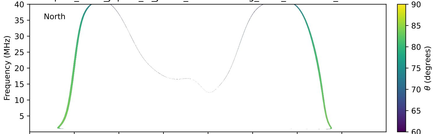
expres_earth_jupiter_io_jrm33_lossc-wid1deg_3kev_19921110_v11.cdf
