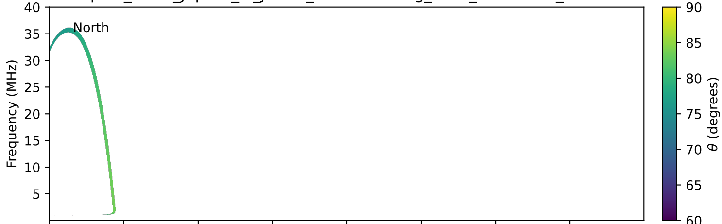
expres_earth_jupiter_io_jrm33_lossc-wid1deg_3kev_19921109_v11.cdf
