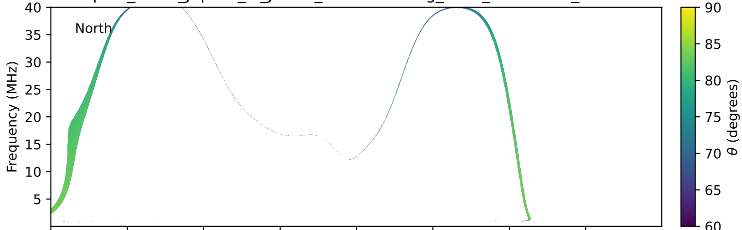
expres_earth_jupiter_io_jrm33_lossc-wid1deg_3kev_19921103_v11.cdf
