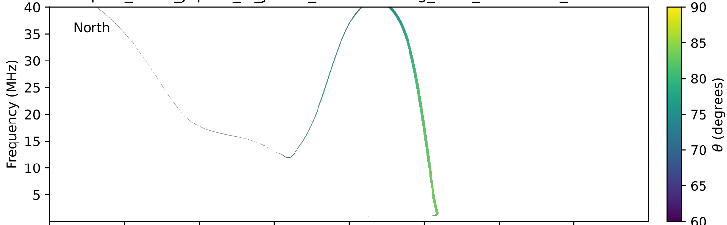
expres_earth_jupiter_io_jrm09_lossc-wid1deg_3kev_19921130_v11.cdf
