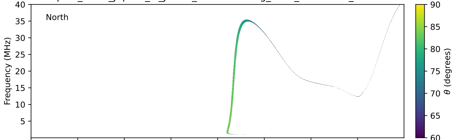
expres_earth_jupiter_io_jrm09_lossc-wid1deg_3kev_19921115_v11.cdf
