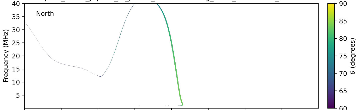
expres_earth_jupiter_io_jrm09_lossc-wid1deg_3kev_19921114_v11.cdf
