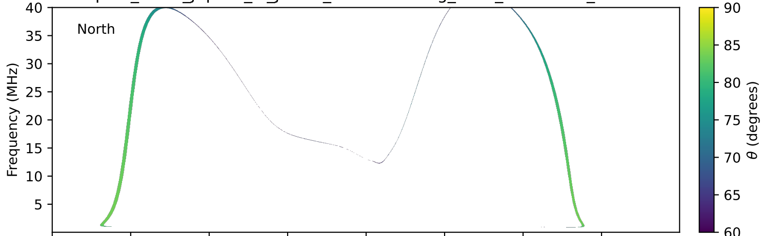
expres_earth_jupiter_io_jrm09_lossc-wid1deg_3kev_19921110_v11.cdf
