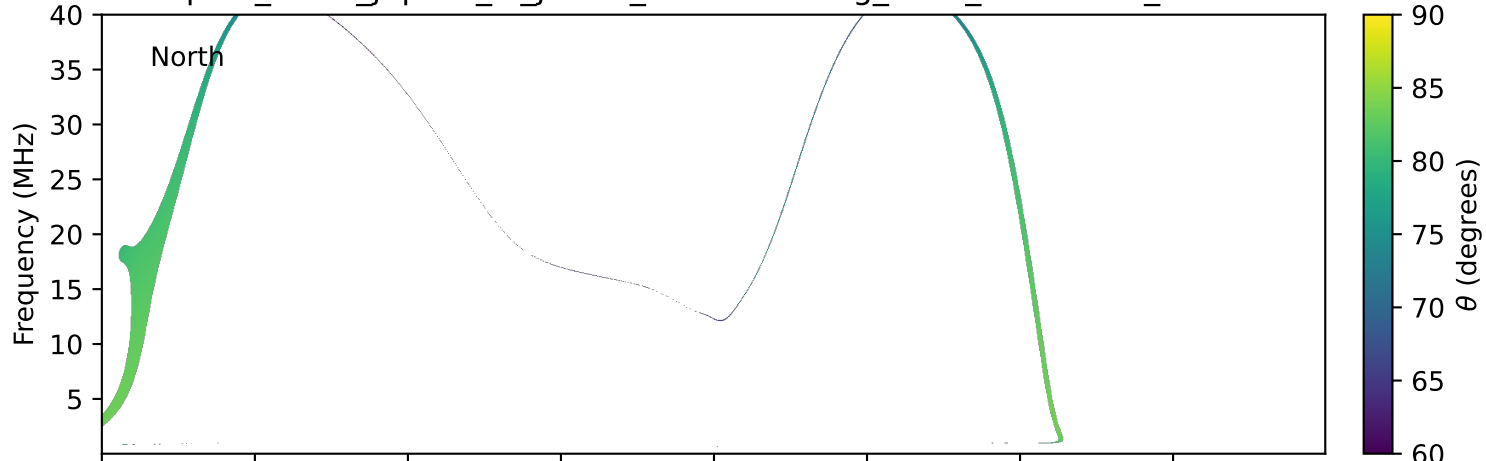
expres_earth_jupiter_io_jrm09_lossc-wid1deg_3kev_19921103_v11.cdf
