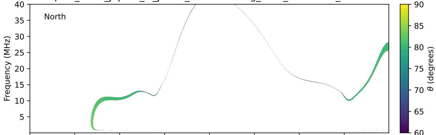
expres_earth_jupiter_io_jrm09_lossc-wid1deg_3kev_19921101_v11.cdf
