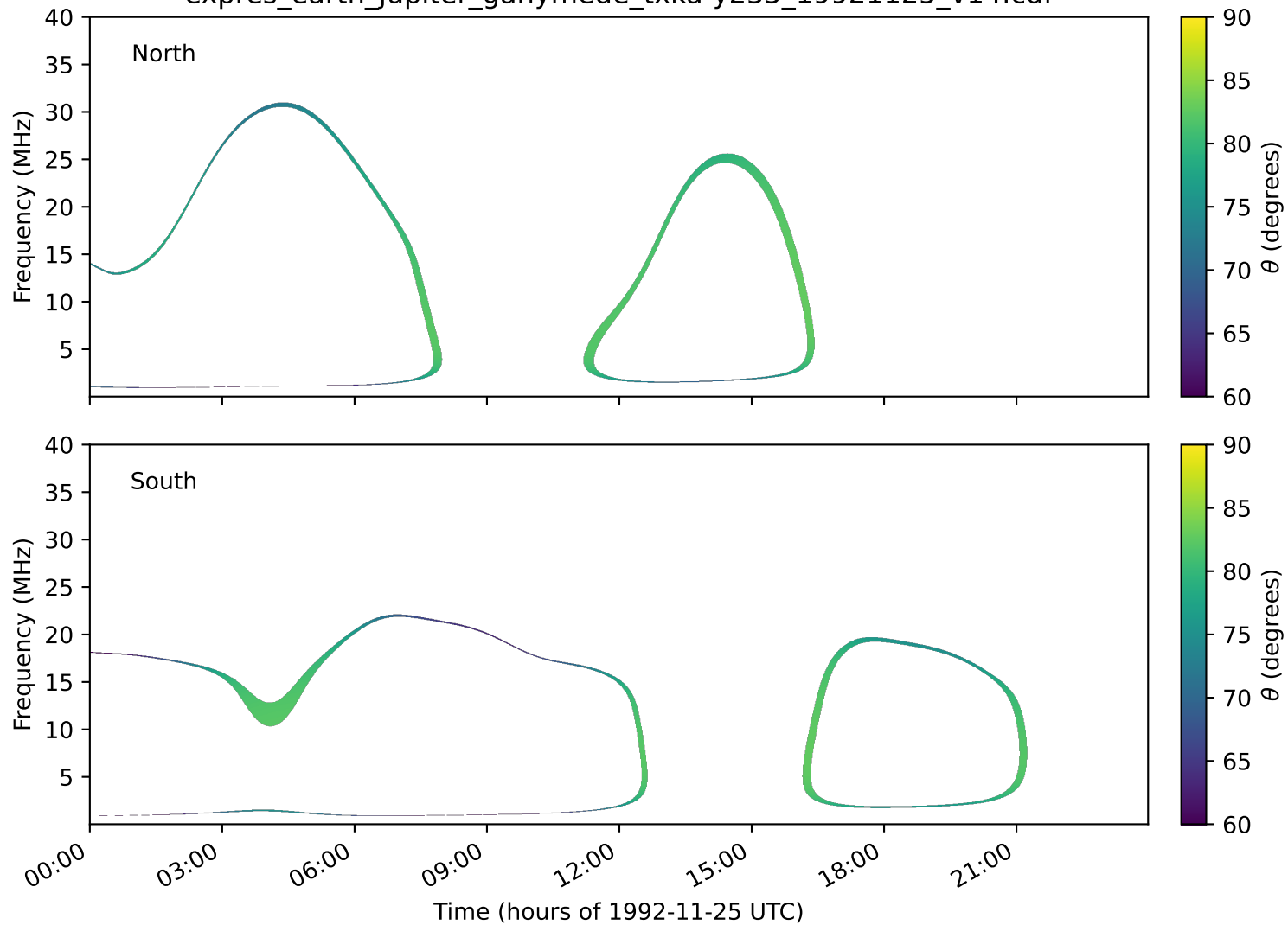
expres_earth_jupiter_ganymede_txka-y235_19921125_v14.cdf
