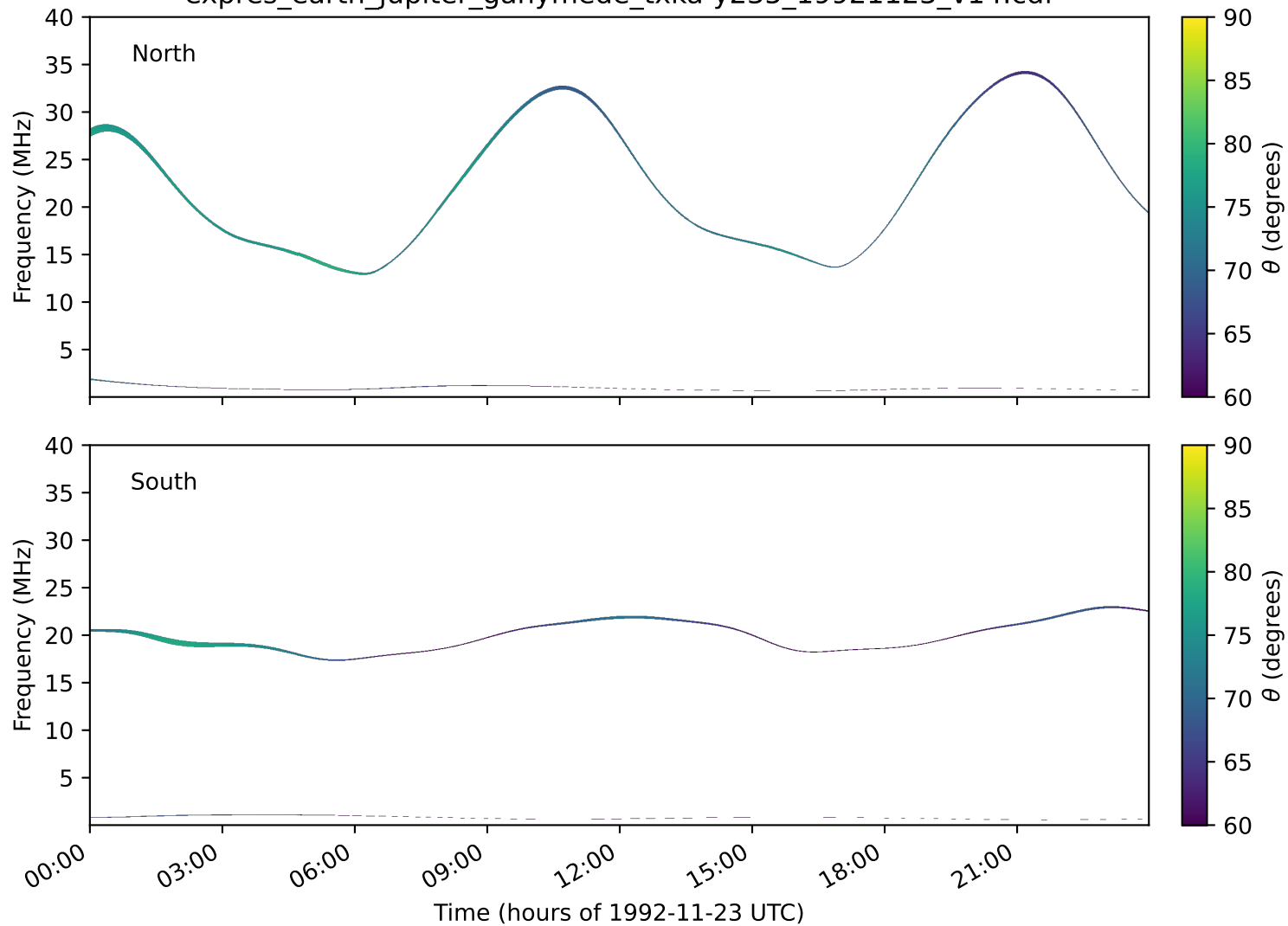
expres_earth_jupiter_ganymede_txka-y235_19921123_v14.cdf
