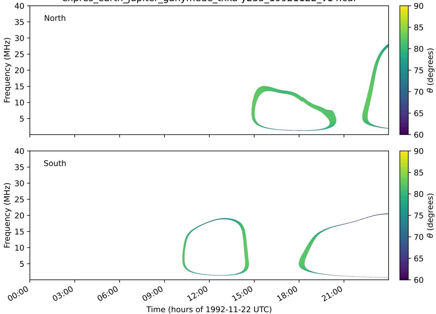
expres_earth_jupiter_ganymede_txka-y235_19921122_v14.cdf
