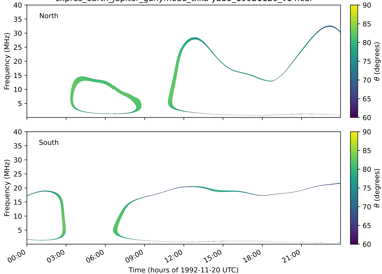
expres_earth_jupiter_ganymede_txka-y235_19921120_v14.cdf
