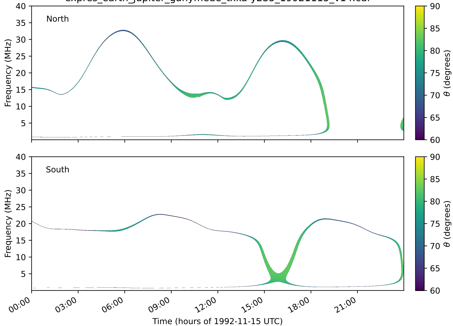
expres_earth_jupiter_ganymede_txka-y235_19921115_v14.cdf
