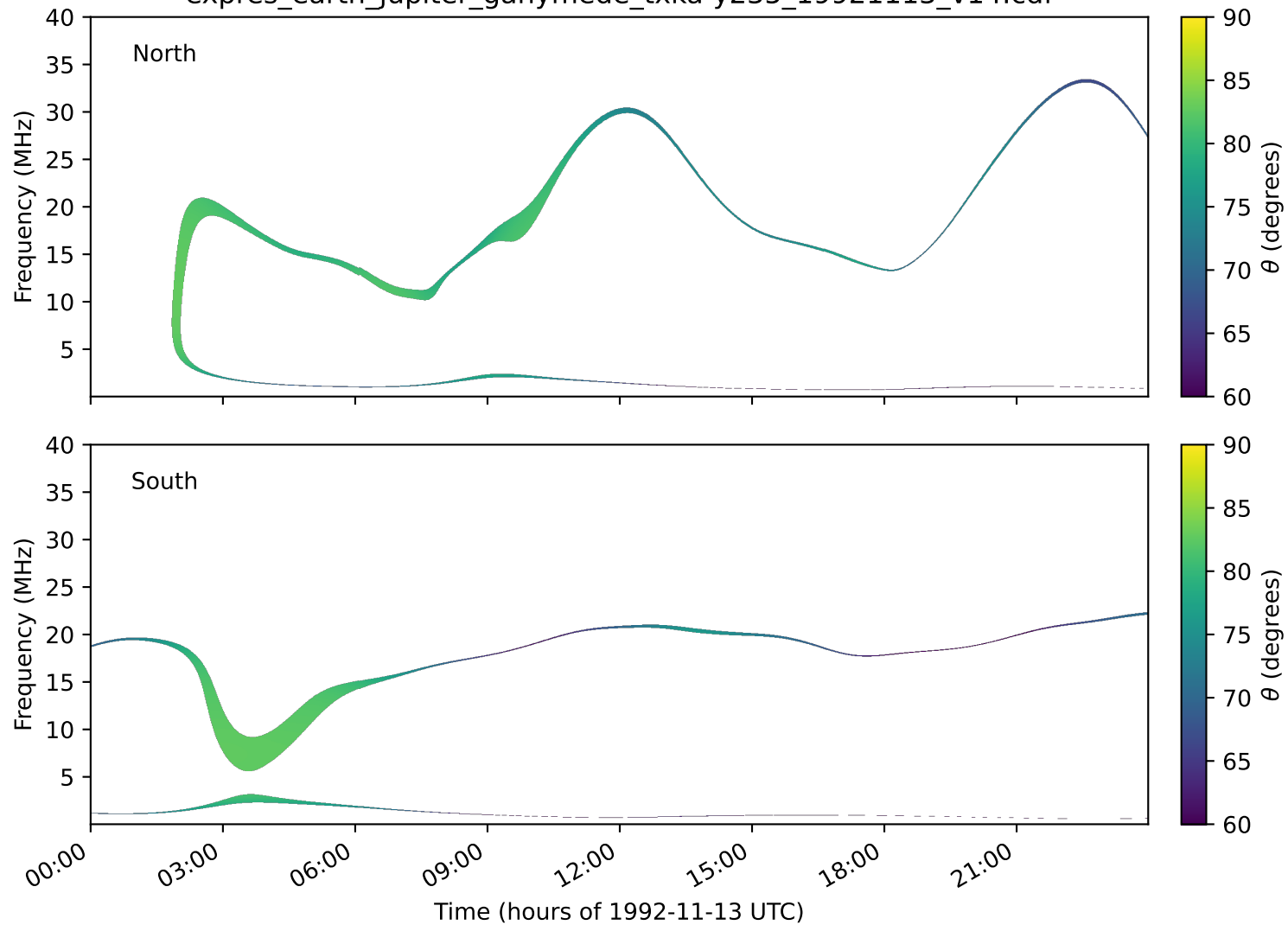
expres_earth_jupiter_ganymede_txka-y235_19921113_v14.cdf
