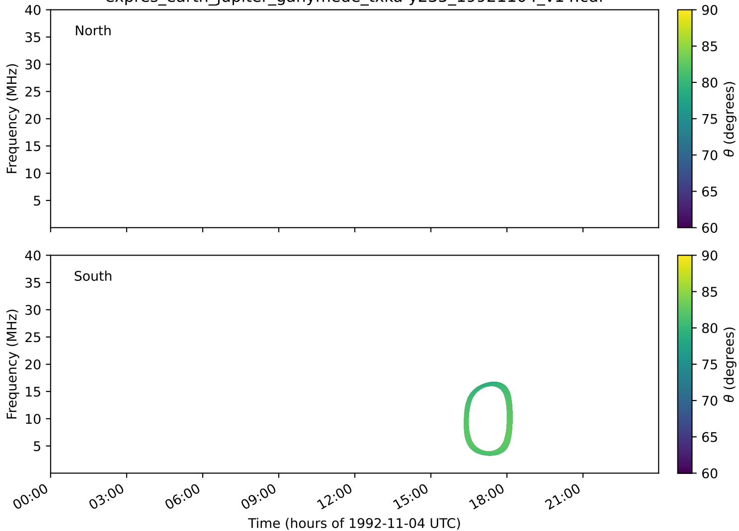
expres_earth_jupiter_ganymede_txka-y235_19921104_v14.cdf
