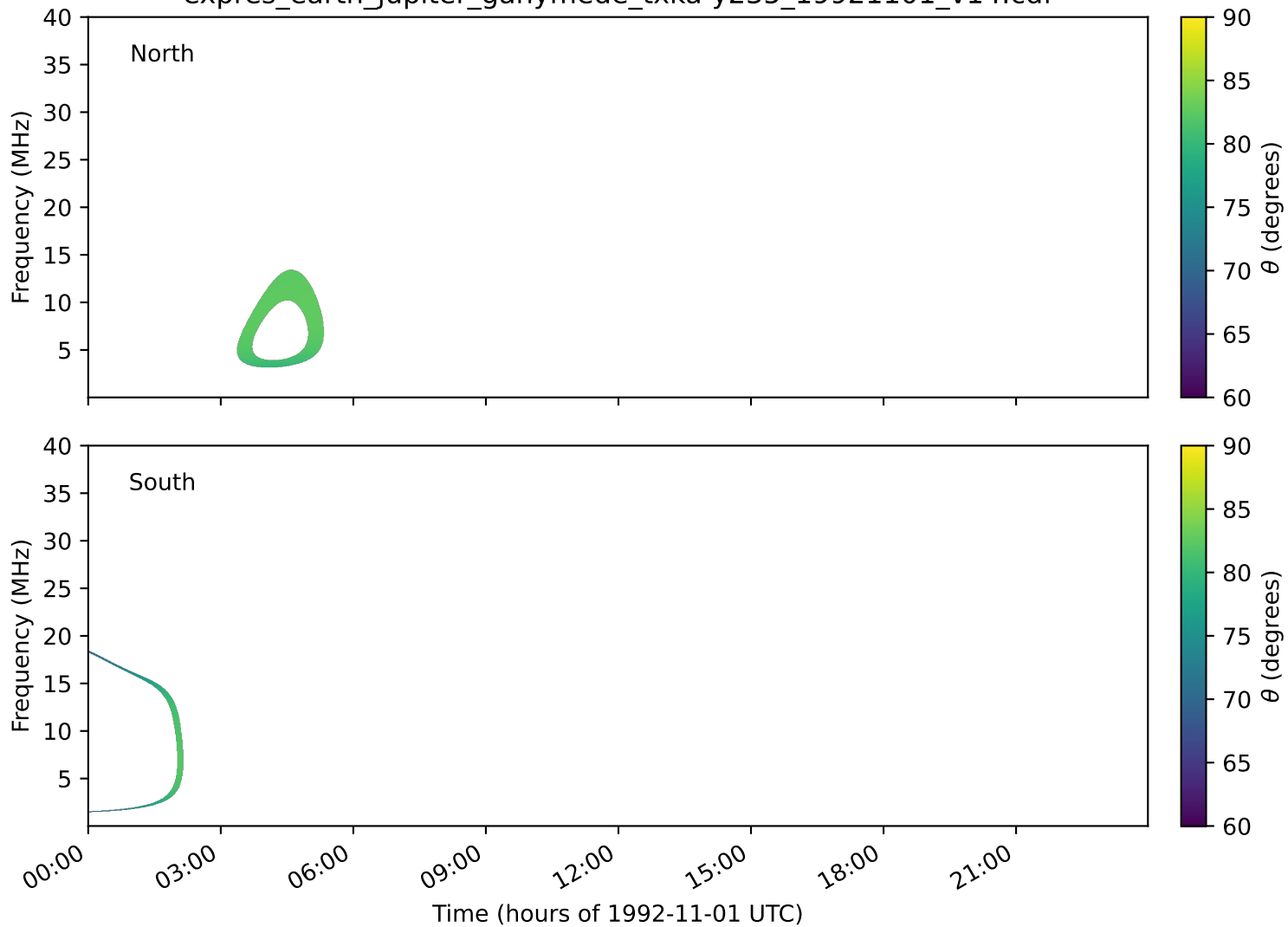
expres_earth_jupiter_ganymede_txka-y235_19921101_v14.cdf
