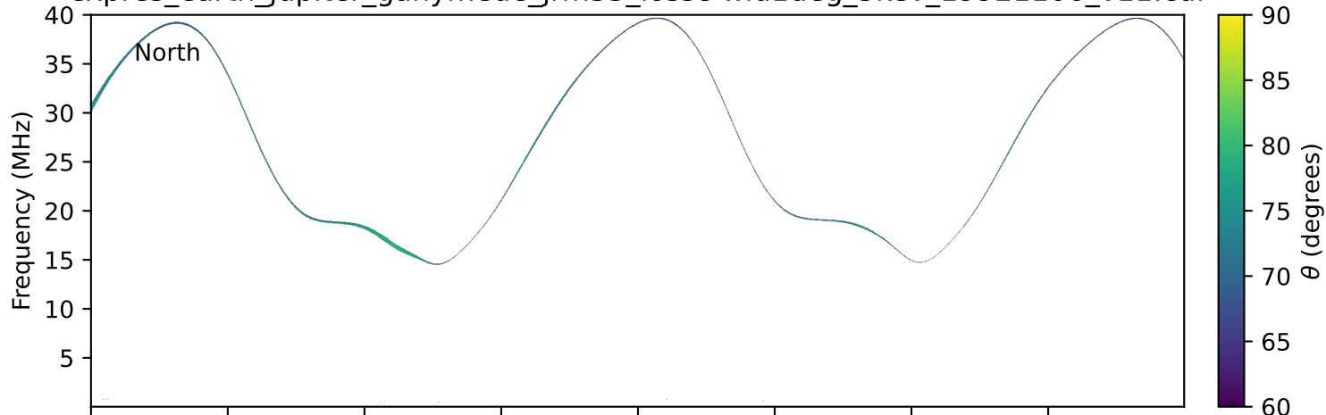
expres_earth_jupiter_ganymede_jrm33_lossc-wid1deg_3kev_19921106_v11.cdf
