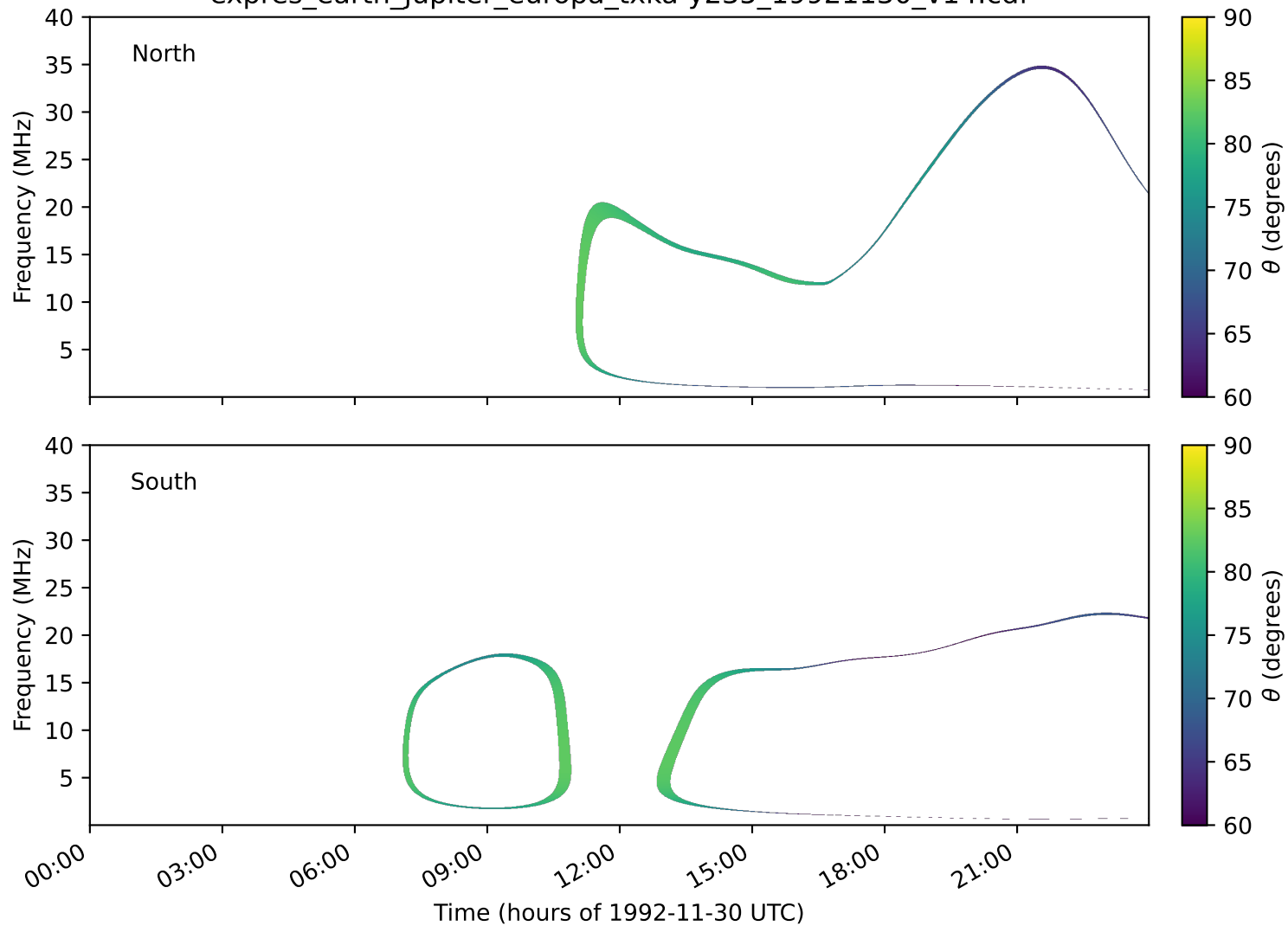
expres_earth_jupiter_europa_txka-y235_19921130_v14.cdf
