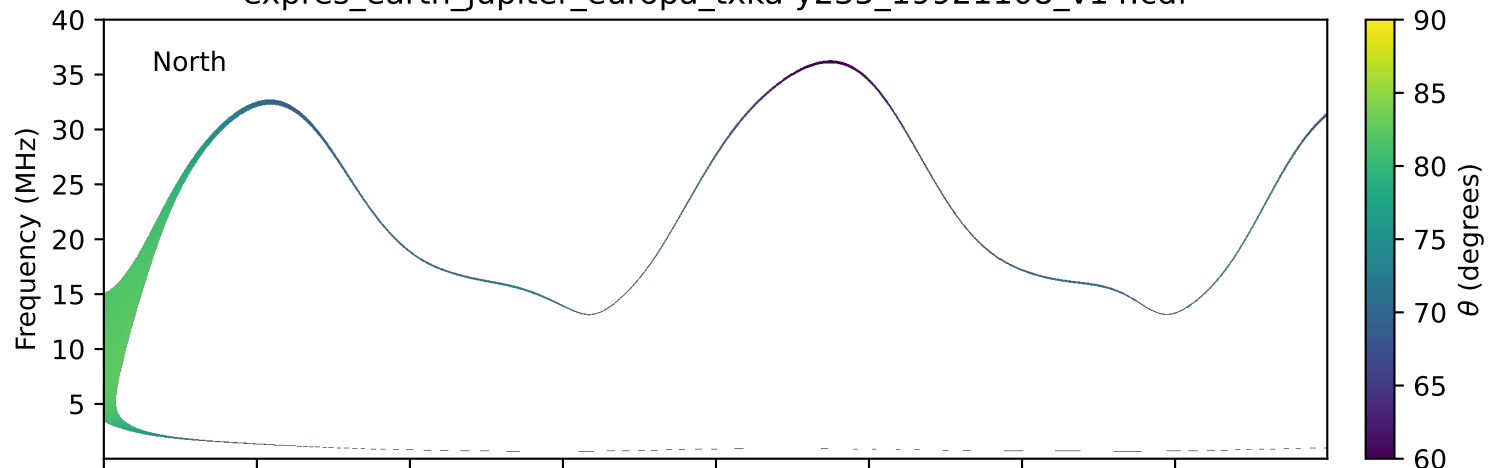
expres_earth_jupiter_europa_txka-y235_19921108_v14.cdf
