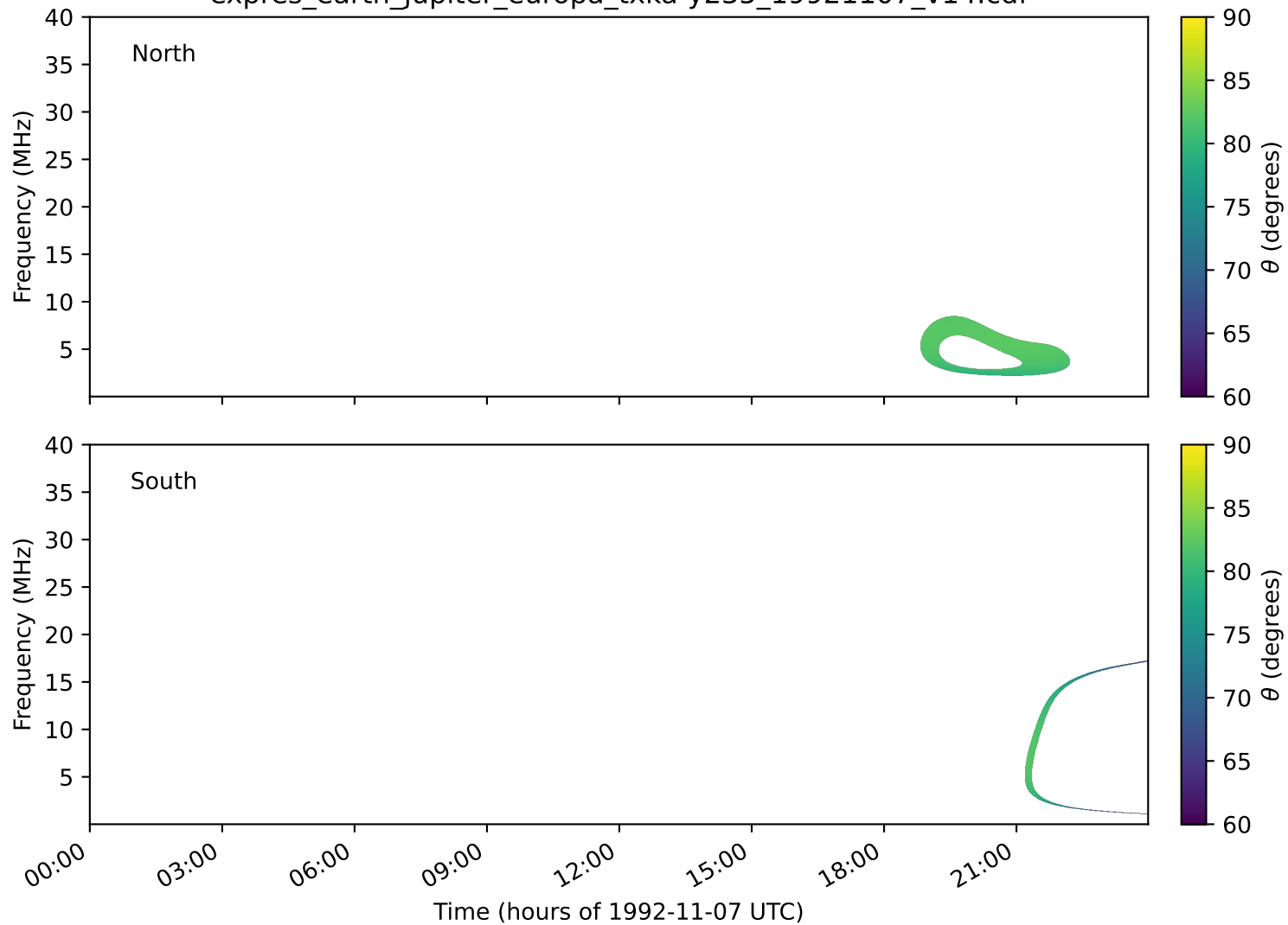
expres_earth_jupiter_europa_txka-y235_19921107_v14.cdf
