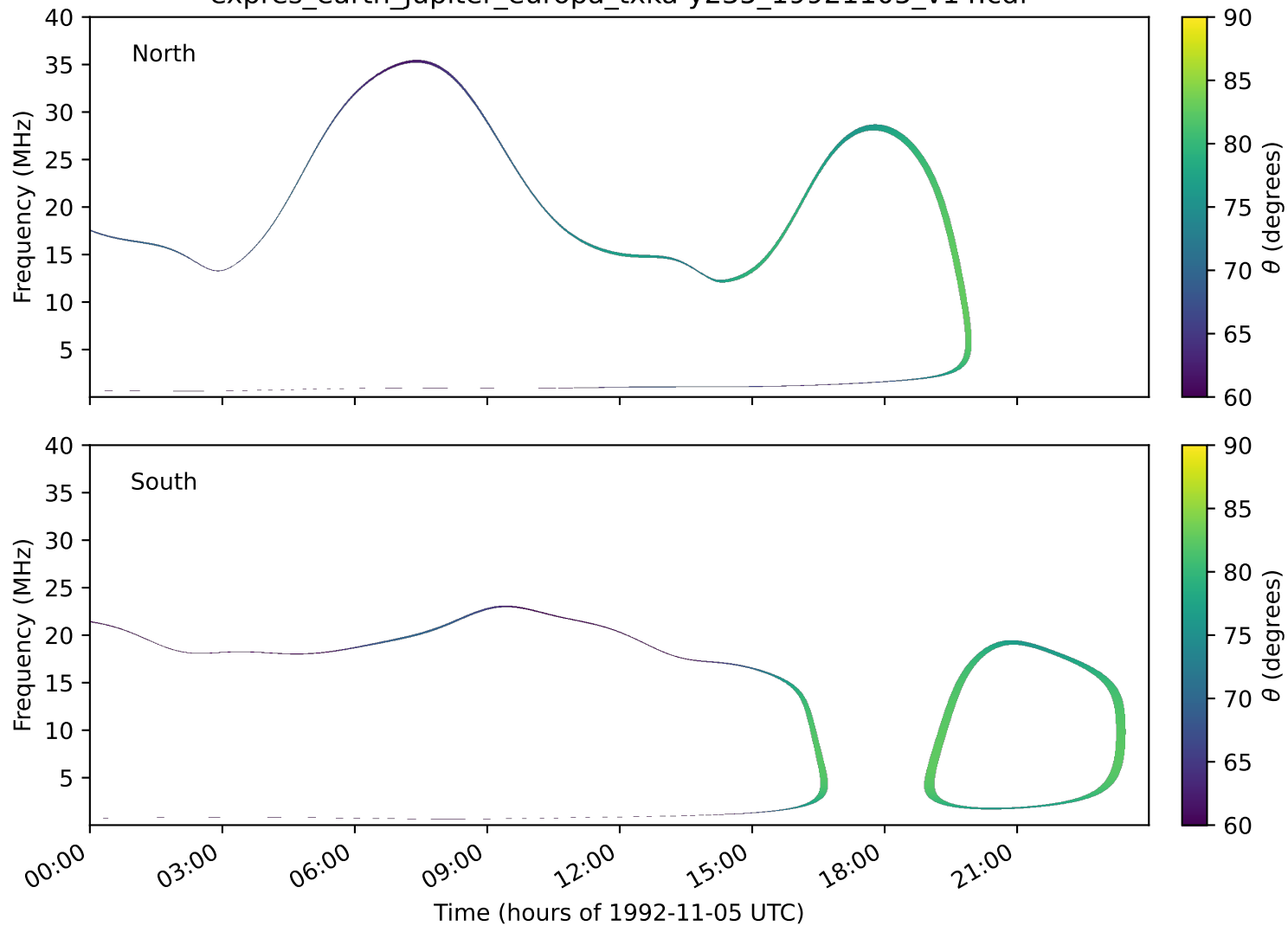
expres_earth_jupiter_europa_txka-y235_19921105_v14.cdf
