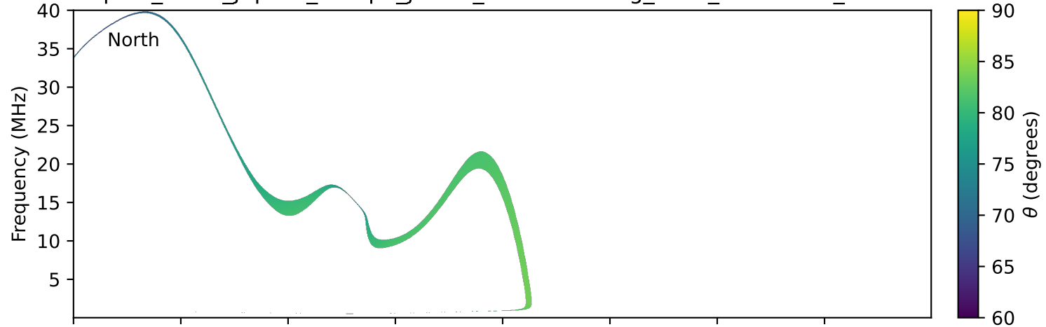
expres_earth_jupiter_europa_jrm33_lossc-wid1deg_3kev_19921128_v11.cdf
