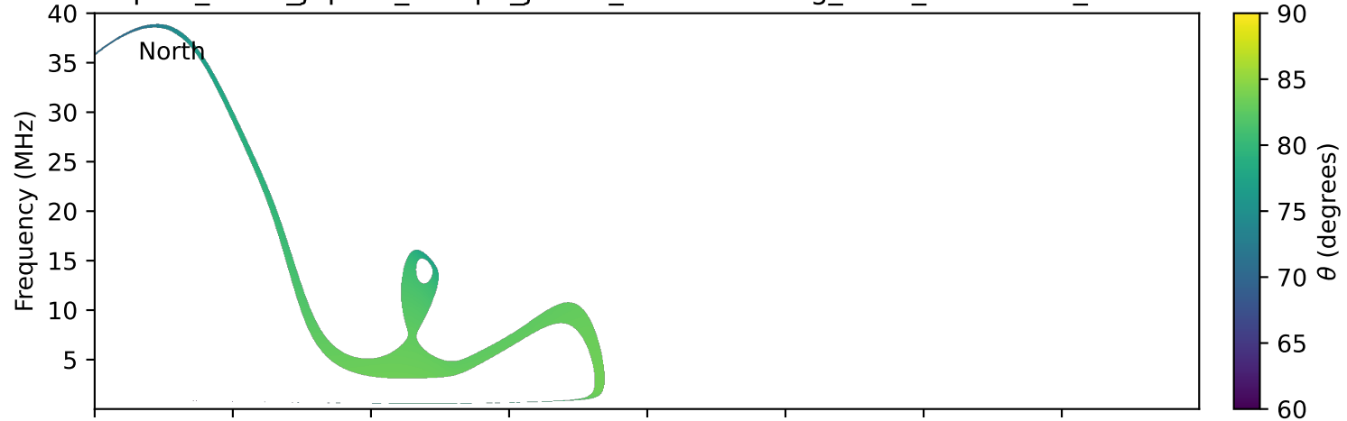
expres_earth_jupiter_europa_jrm33_lossc-wid1deg_3kev_19921121_v11.cdf
